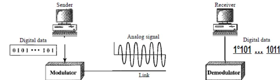
Figure 5.1 Digital-to-analog conversion
