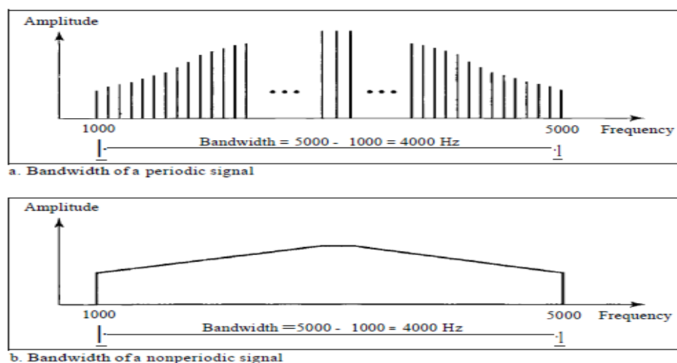
Figure 3.12 The bandwidth of periodic and nonperiodic composite signals
